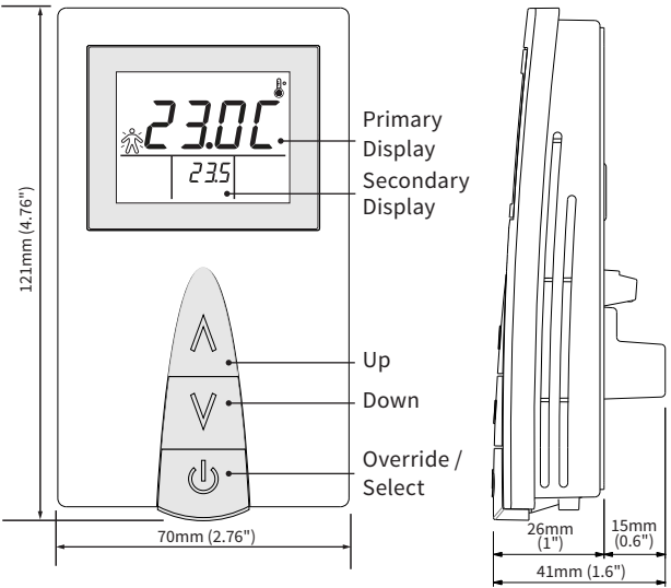
SENW5x Dimensions and Identification (SENW58C Shown)
