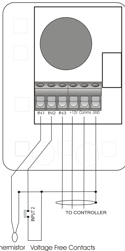
Rear View of Control Station
