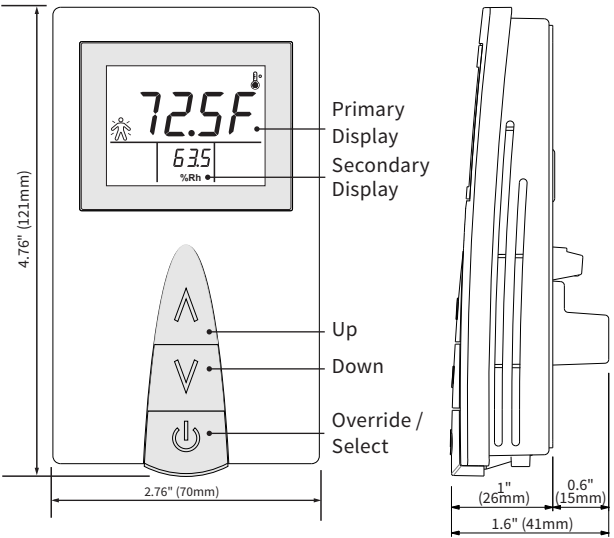
HTW5x Dimensions and Identification (HTW58F shown)
